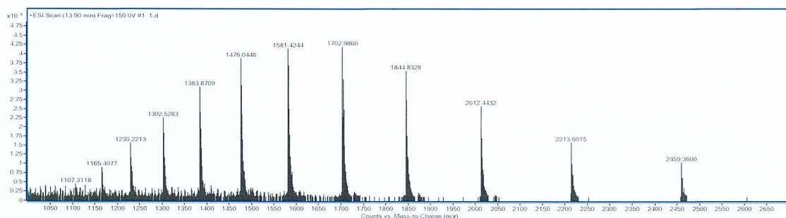
Figure 4 – Mass-spectrum of the test sample, RT= 13,93 min.
